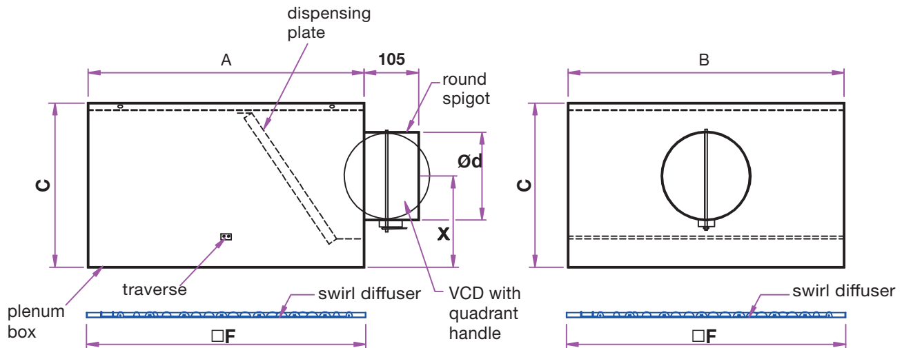
SQUARE TYPE WITH PLENUM BOX & VCD AT SIDE SPIGOT: MODEL SW3SRIDPSV
