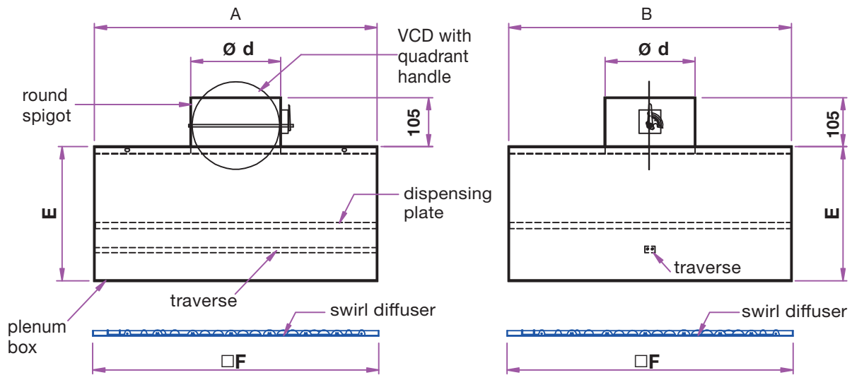
SQUARE TYPE WITH PLENUM BOX & VCD AT TOP SPIGOT: MODEL SW3SRIDPTV
